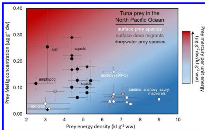
Figure 1. Energy density ( \text{kJ g}^{-1} \text{ww} ), methylmercury ( \text{MeHg} ) concentrations ( \mu\text{g g}^{-1} \text{dw} ), and depth distribution of pelagic prey in the eastern (circles) and western (diamonds) North Pacific Ocean. Symbols show means (error bars \pm 1 \text{ SD} ) for surface foraging fish, diel-vertically migrating, and deepwater (mesopelagic and bathypelagic) prey. Prey energy densities are based on literature values (SI Table S2).
